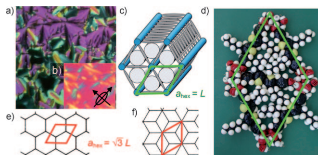
Figure 3. Triangular cylinder phase (Col hex /p6mm) of compound 2 (6,6). a) Texture between crossed polarizers at T = 70 °C; the dark areas represent homeotropically aligned regions. b) Texture with \lambda retarder plate and indicatrix; in the fans the high-index axis is radial; since the columns are tangential in the fans the high-index axis is perpendicular to the columns. [13] c, d) Model showing the organization of the molecules; the hexagonal lattice (green) coincides with the cylinder walls formed by the \pi -conjugated rodlike cores. e, f) Alternative hexagonal lattices (red) formed by hexagonal or rhombic cylinders which would give much larger lattice parameters ( L = molecular length).
