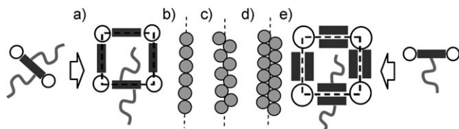
Figure 4. Dependence of wall thickness on the number of lateral chains, shown for square honeycomb phases; a,e) cuts through one cylinder; b–d) cuts through a cylinder wall along the cylinder axis. a,b) Single-wall structure of X-shaped bolaamphiphiles; c) staggered organization of the aromatic cores as in 2 (12,12), and d,e) double-wall cylinders of the T-shaped molecule 1 (12,0).
