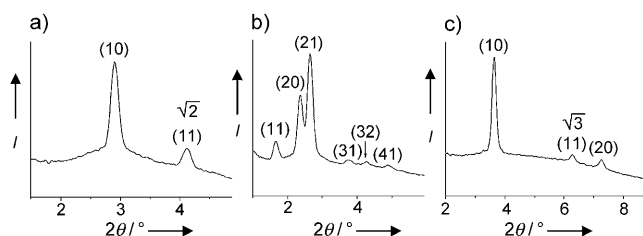
Figure 2. SAXS powder pattern of a) 1 (12,0) at 143 °C (Col squ /p4mm); b) 1 (18,0) at 150 °C (Col squ /p4gm); c) 2 (6,6) at 70 °C (Col hex /p6mm) with indexation.
