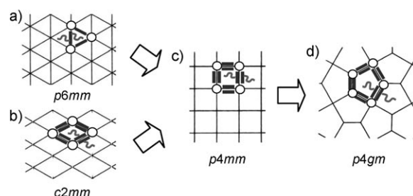
Figure 1. Tiling patterns and their 2D lattices; the views result from cuts through the self-assembled LC polygonal honeycomb phases perpendicular to the cylinder long axis (white dots: columns incorporating the H-bonding networks, bold lines: aromatic cores). a) A triangle honeycomb formed by the X-shaped bolaamphiphile 2/6 and b–d) tilings with rhombuses, squares, and pentagons, as reported previously for T-shaped bolaamphiphiles. [2,3]
